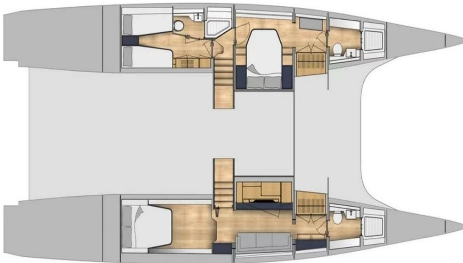
3 CABIN LAYOUT
