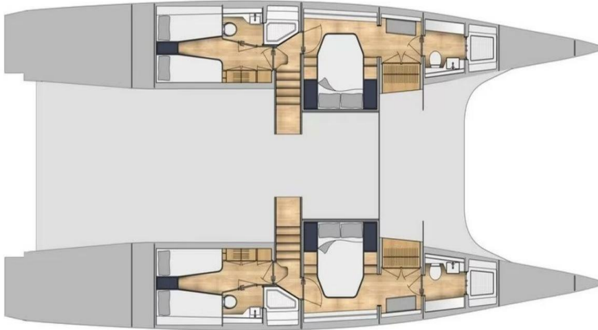
4 CABIN LAYOUT
