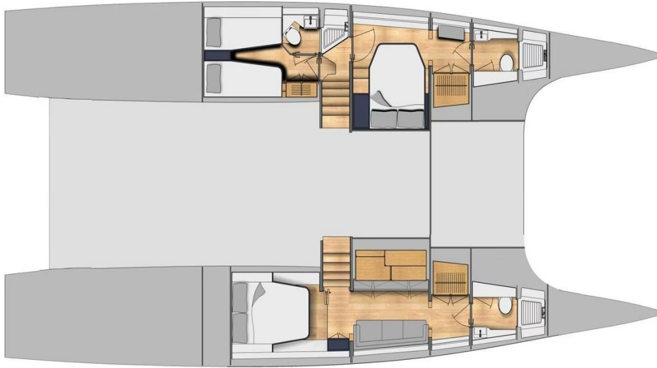
3 CABIN LAYOUT
