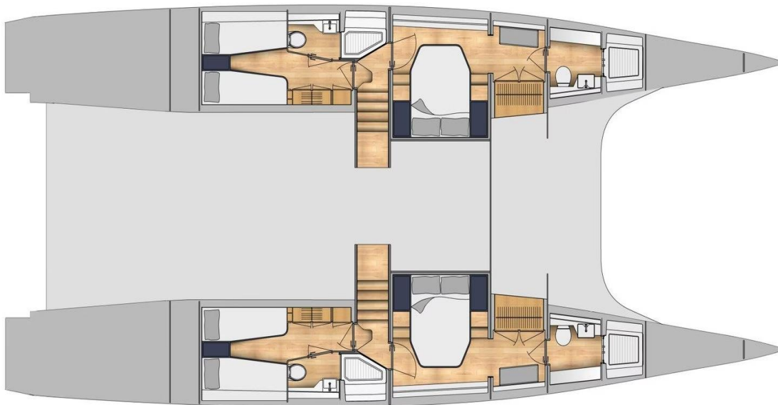
4 CABIN LAYOUT
