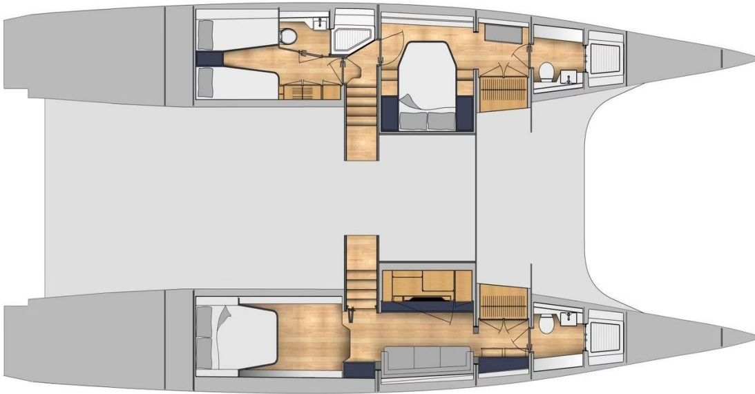
3 CABIN LAYOUT
